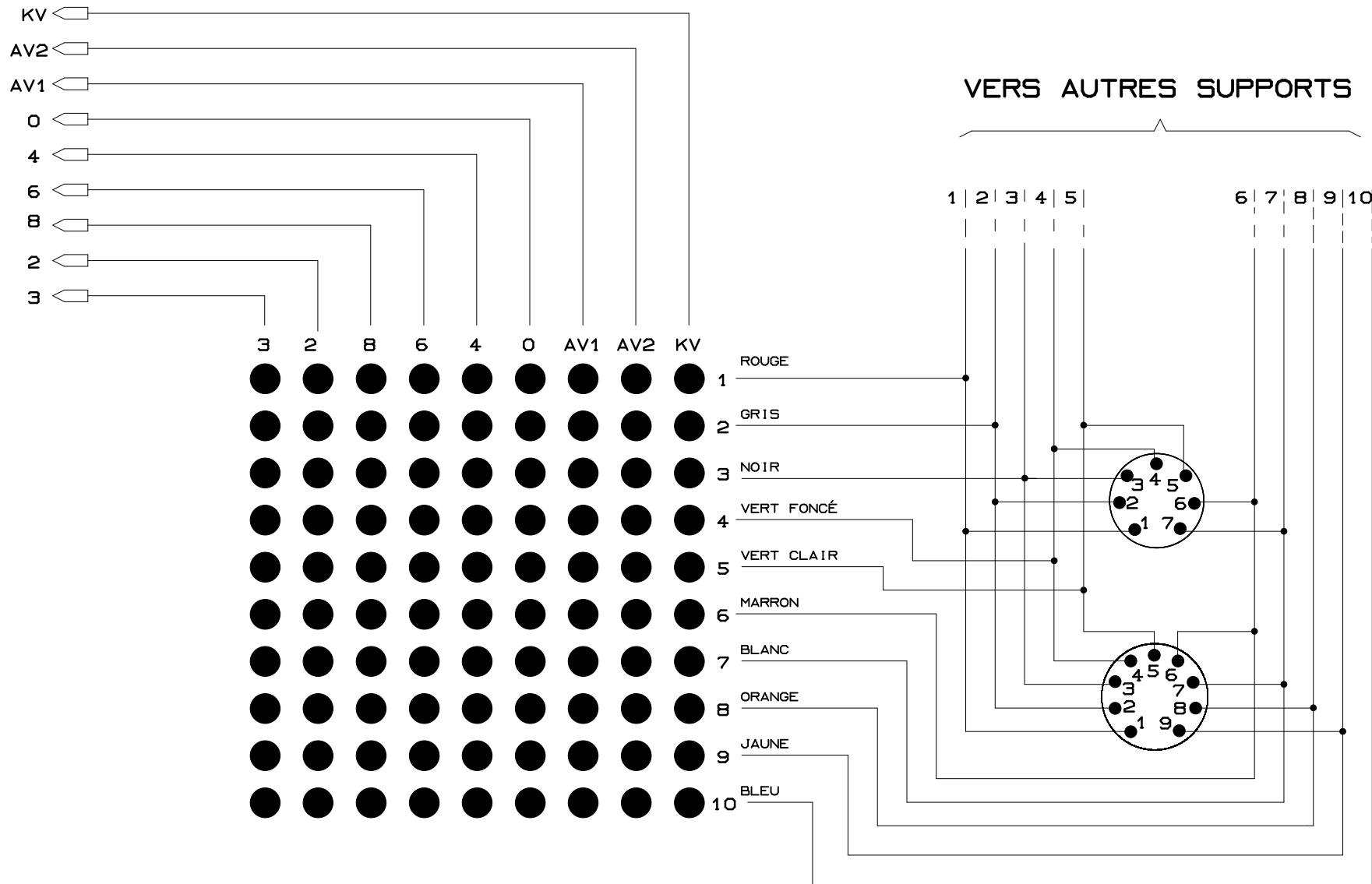
LAMPOMETRE FC2008 CABLAGE 3
